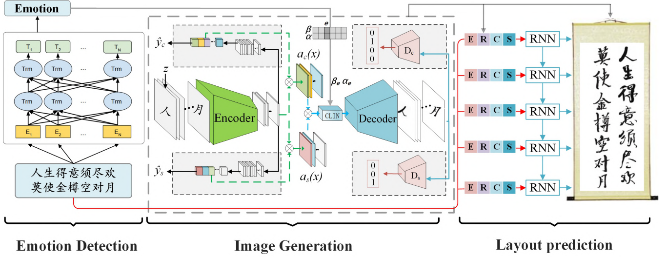
Figure 2: Overview of our emotional calligraphy generation framework.
